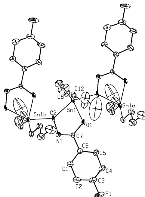
Figure 1. Diagram of a section of polymeric 1 . Hydrogen atoms are omitted for clarity.
