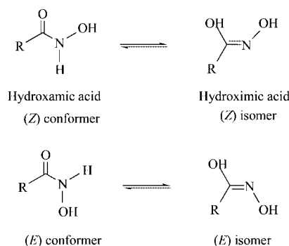
Scheme 1. Isomers of hydroxamic acids.
