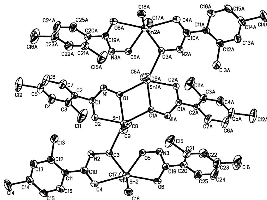
Figure 3. Diagram of the dimeric repeating units in polymeric 3 . Hydrogen atoms are omitted for clarity.
