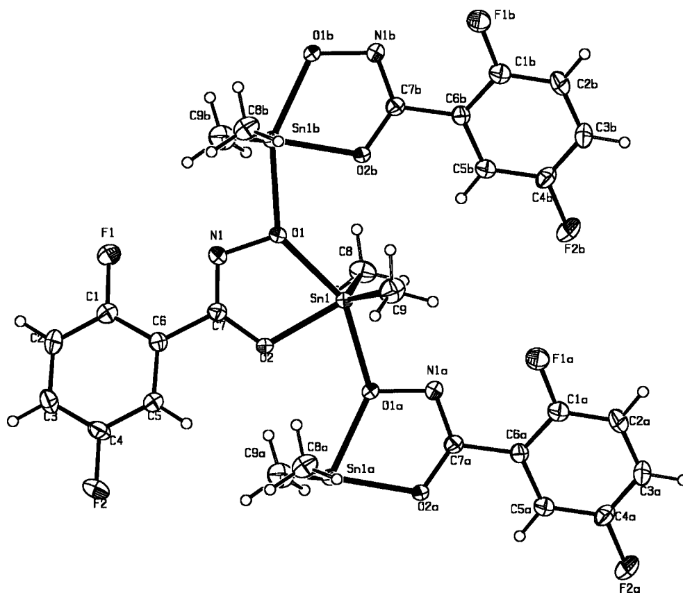
Figure 2. ORTEP drawing of a section of polymeric 2 with atomic numbering scheme.
