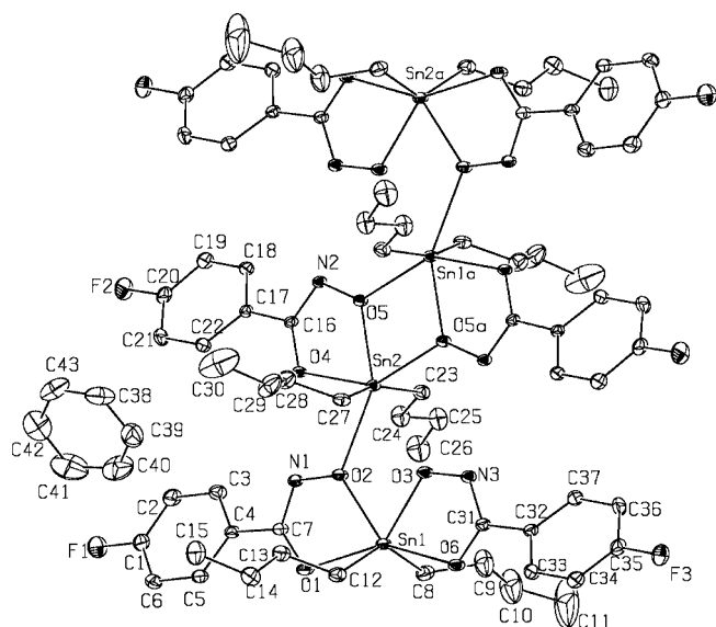
Figure 4. Diagram of the dimeric repeating units in polymeric 4 . Hydrogen atoms are omitted for clarity.
